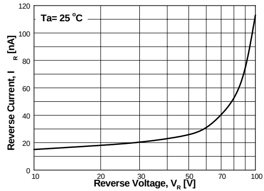
GENERAL RULE: The Reverse Current of a diode will approximately double for every ten (10) Degree C increase in Temperature Figure 2. Reverse Current vs Reverse Voltage IR - 10 to 100V
